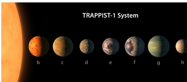
An artist's illustration of the seven Earth-sized worlds of the Trappist-1 system.
