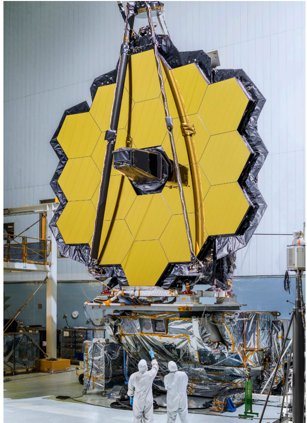
The primary mirror of the James Webb Space Telescope during testing at NASA's Goddard Space Flight Center.
