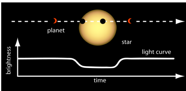
As an exoplanet passes in front of a star, it blocks some of the starlight in a mini-eclipse.
