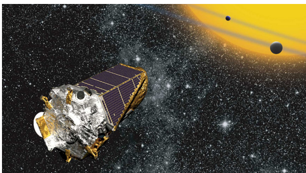
NASA's Kepler mission has discovered over 2,000 exoplanets using the transit method since its launch in 2009.
